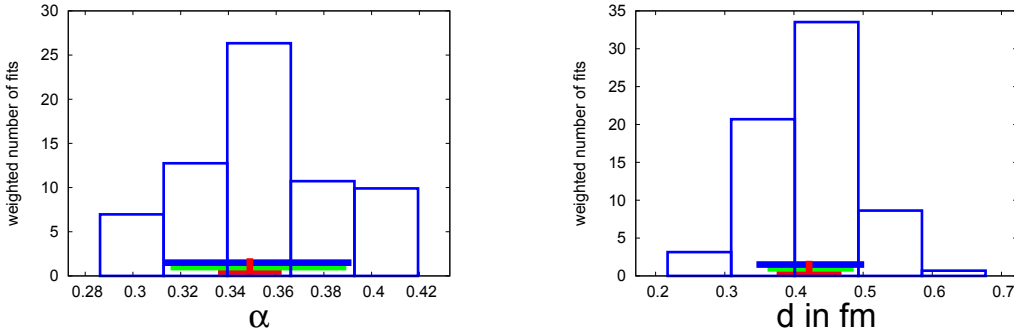
Figure 1: Histograms for the scalar isosinglet for qq = ud . The red/green/blue bars indicate the statistical/systematic/combined errors.
