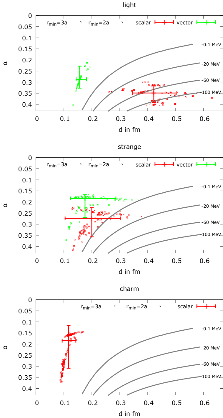
Figure 3: Binding energy isolines E_B = \text{constant} in the \alpha - d -plane for u/d , s and c light quarks qq together with the fit results of eq. (4.1) to lattice potentials.
