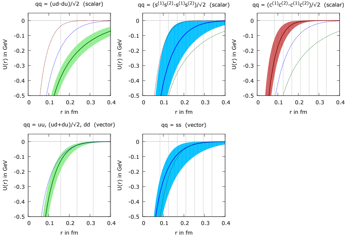
Figure 2: Potentials fits for different channels (upper line: scalar isosinglet; lower line: vector isotriplet). The curves without an error band are copied from the respective other plots in the same line for easy comparison. Vertical lines indicate the available lattice \bar{b}b separations.
