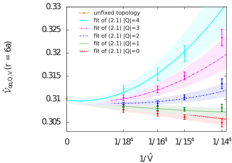
Fig. 1. \hat{\mathcal{V}}_{q\bar{q},Q,V}(r=6a) as a function of 1/\hat{V} . The curves represent the fit of the lattice static potential results to eq. (2.1).
