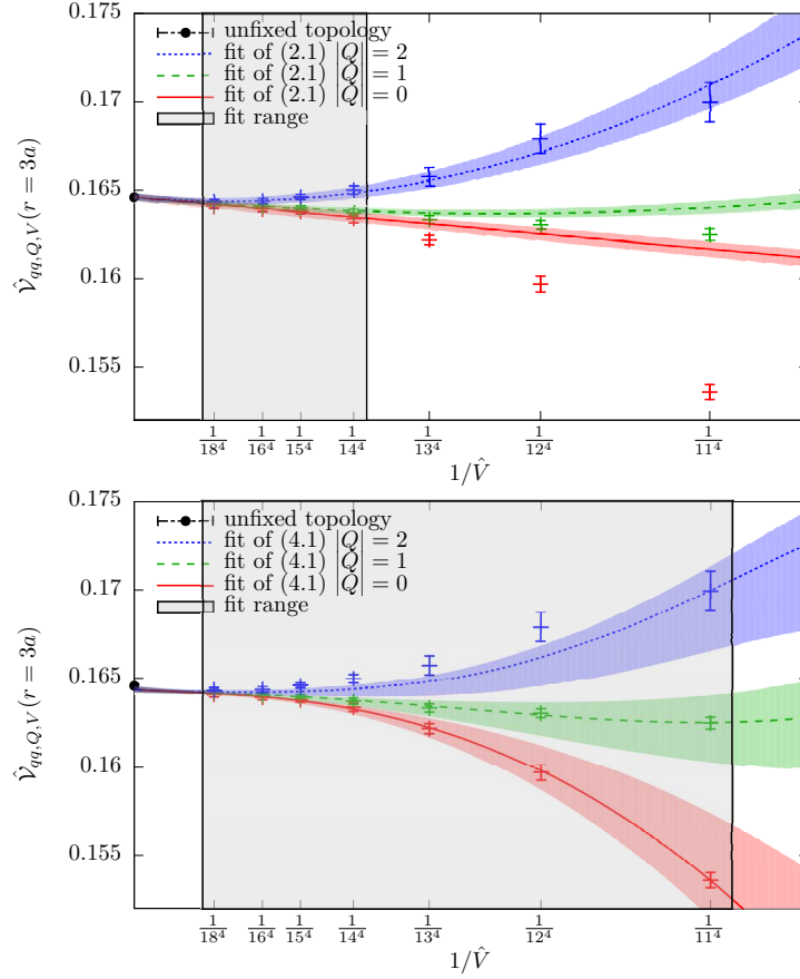
Fig. 3. \hat{\mathcal{V}}_{q\bar{q},Q,V}(r=3a) as a function of 1/\hat{V} . (top): The curves represent the fit of eq. (2.1) to the lattice static potential results for large volumes \hat{V} = 14^4, 15^4, 16^4, 18^4 . There is a strong discrepancy between these curves and the lattice results for the small volumes \hat{V} = 11^4, 12^4, 13^4 . (bottom): The curves represent the fit of eq. (4.1) to the lattice static potential results for all volumes \hat{V} = 11^4, \dots, 18^4 . There is almost perfect agreement, even at small volumes and Q = 0 .
