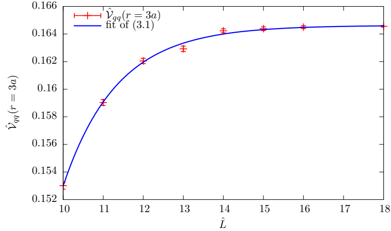
Fig. 2. The dependence of \hat{\mathcal{V}}_{q\bar{q}}(r=3a) on the periodic spatial extension \hat{L} of the lattice (at unfixed topology).
