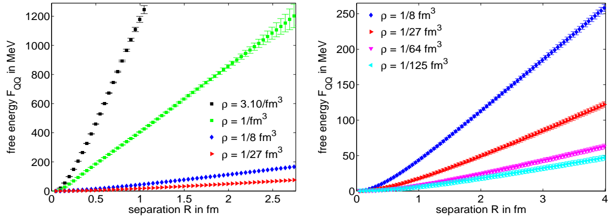
Figure 6: The free energy of a pair of static charges F_{Q\bar{Q}} as a function of the separation R for various dyon densities \rho .
