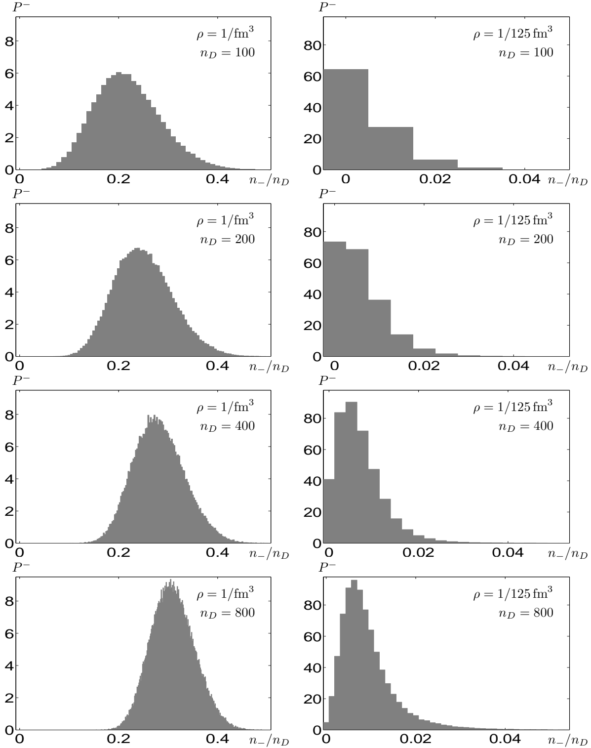
Figure 1: Histograms obtained from 100,000 independently chosen dyon configurations representing the probability distribution P^-(n_-) of the number of negative eigenvalues (as function of n_-/n_D ). Left column: \rho = 1/\text{fm}^3 . Right column: \rho = 1/125 \text{ fm}^3 .
