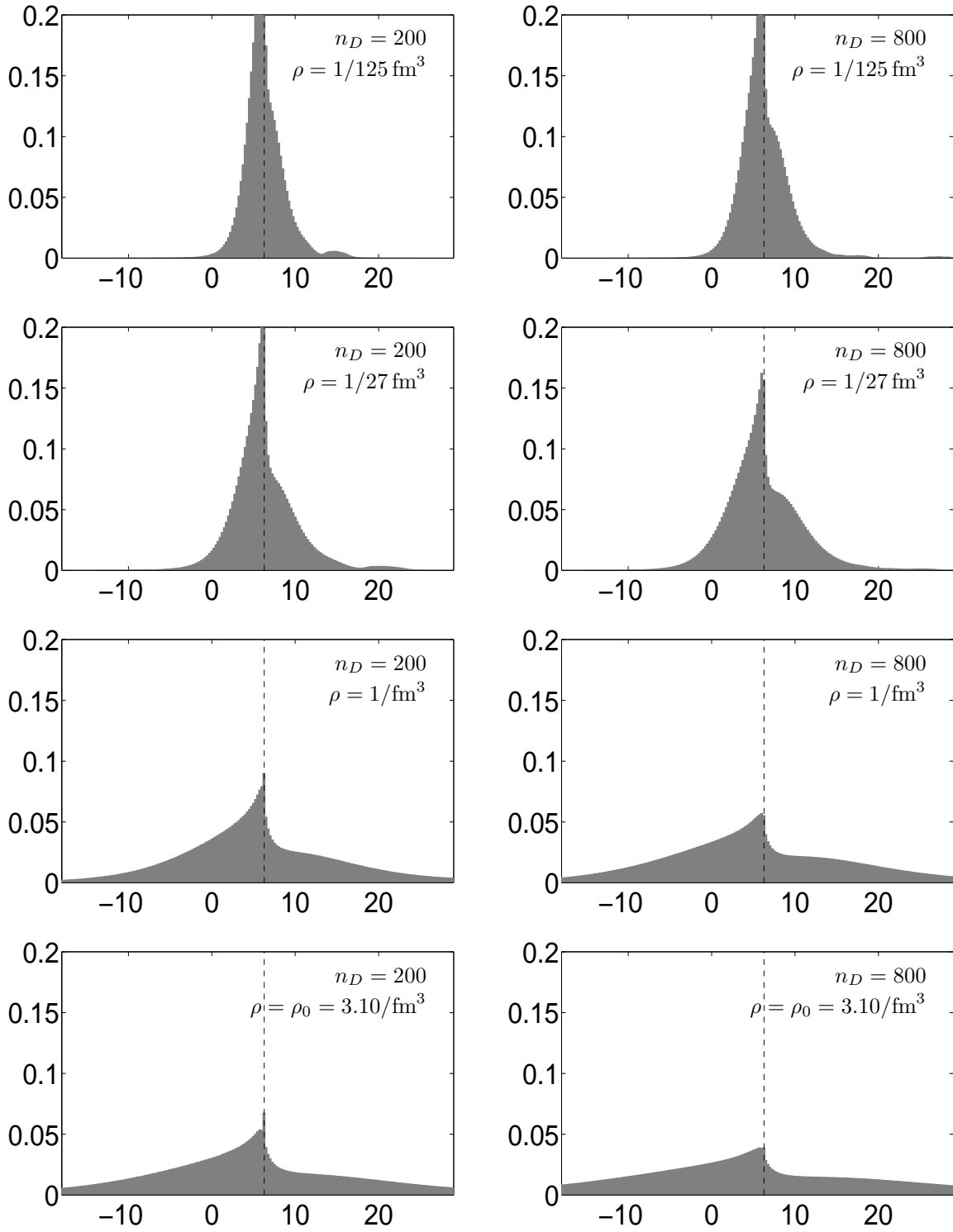
Figure 4: Histograms obtained from 100,000 independently chosen dyon configurations representing the spectral density of the approximate moduli space metric G . Left column: n_D = 200 . Right column: n_D = 800 .
