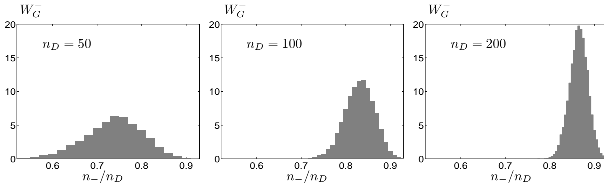
Figure 2: Integrated weights W_G^-(n_-) (shown as functions of n_-/n_D ) for various dyon numbers n_D and a fixed density \rho = 1/\text{fm}^3 .
