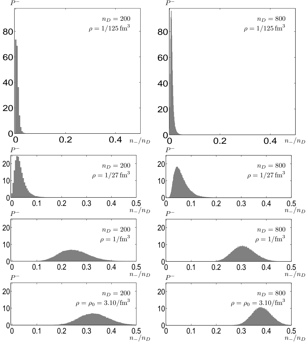
Figure 3: Histograms obtained from 100,000 independently chosen dyon configurations representing the probability distribution P^-(n_-) of the number of negative eigenvalues (as function of n_-/n_D ). Left column: n_D = 200 . Right column: n_D = 800 .
