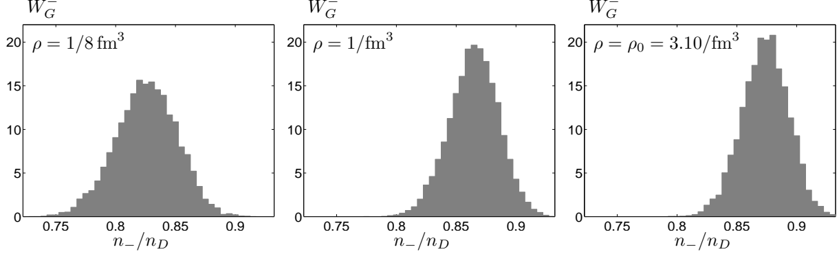
Figure 5: Integrated weights W_G^-(n_-) , shown as functions of n_-/n_D , as obtained for a number n_D = 200 of dyons and various densities.
