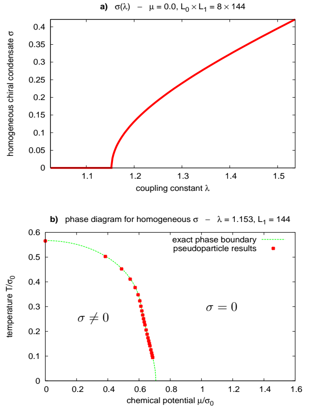
FIG. 4: Q^\dagger Q -regularization, L_1 = 144 . a) \mu = 0.0 , L_0 = 8 . \sigma as a function of \lambda . b) \lambda = 1.153 . The pseudoparticle phase diagram for homogeneous chiral condensate together with the exact phase boundary.
