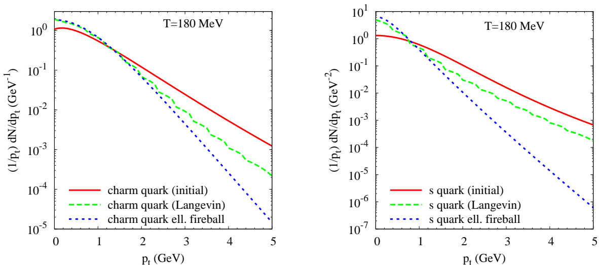
FIG. 2: (Color online) Quark p_t distributions resulting from relativistic Langevin simulations of an expanding elliptic QGP fireball at the end of a QGP (mixed) phase at a temperature of T = 180 MeV and average radial surface expansion velocity, \langle\beta_0\rangle \simeq 0.48c . The numerically computed spectra (long-dashed lines) are compared to the initial spectra (solid lines) and to a blast-wave parameterization for particles with the same mass and the same fireball conditions ( T = 180 MeV and the same flow field as used for the background medium in the Langevin simulation; short-dashed lines). Left and right panels correspond to charm ( m_c = 1.5 GeV) and strange ( m_s = 0.45 GeV) quarks, respectively.
