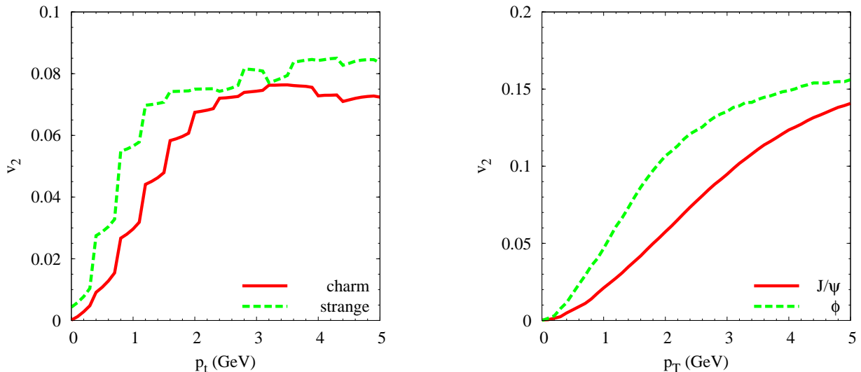
FIG. 5: (Color online) Elliptic flow coefficient, v_2 , as a function of transverse momentum for c and s quarks (left panel), as well as J/\psi and \phi mesons resulting from quark recombination (right panel), in semicentral \sqrt{s_{NN}} = 200 GeV Au-Au collisions.
