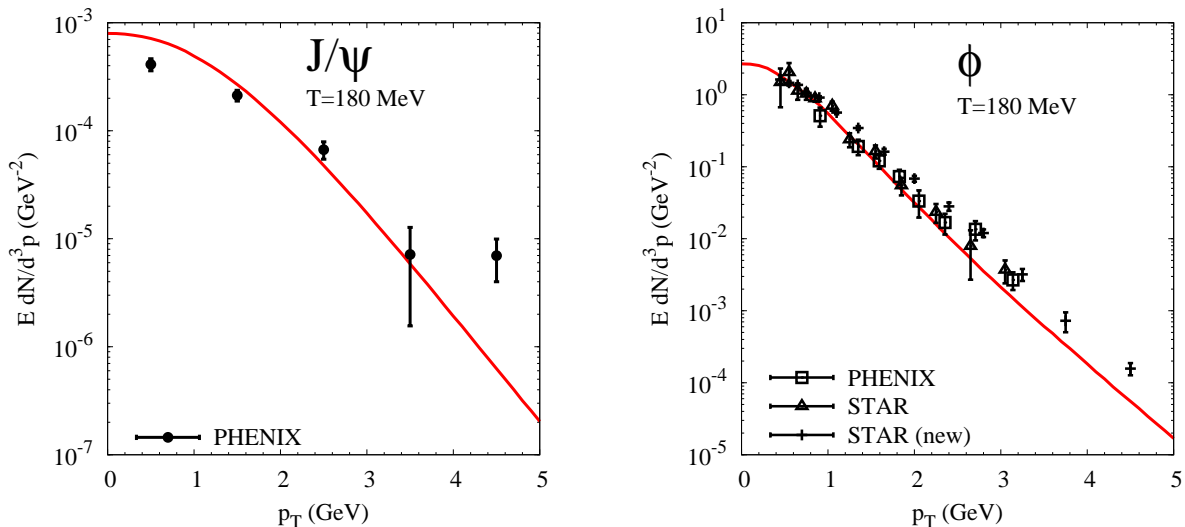
FIG. 3: (Color online) Meson p_T spectra from quark-antiquark coalescence in central \sqrt{s_{NN}} = 200 GeV Au-Au collisions computed within the resonance recombination model for J/\psi (left panel) and \phi (right panel); experimental data are from Refs. [36] and [37–39], respectively.
