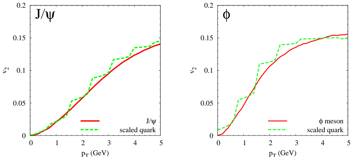
FIG. 4: (Color online) Scaled quark v_2^{\text{scaled}} (dashed lines) and meson v_{2,M} (solid lines) coefficients as a function of meson p_T for J/\Psi ( Q = 0.1 GeV, \Gamma = 0.1 GeV; left panel) and \phi ( Q = 0.12 GeV, \Gamma = 0.05 GeV; right panel) mesons.
