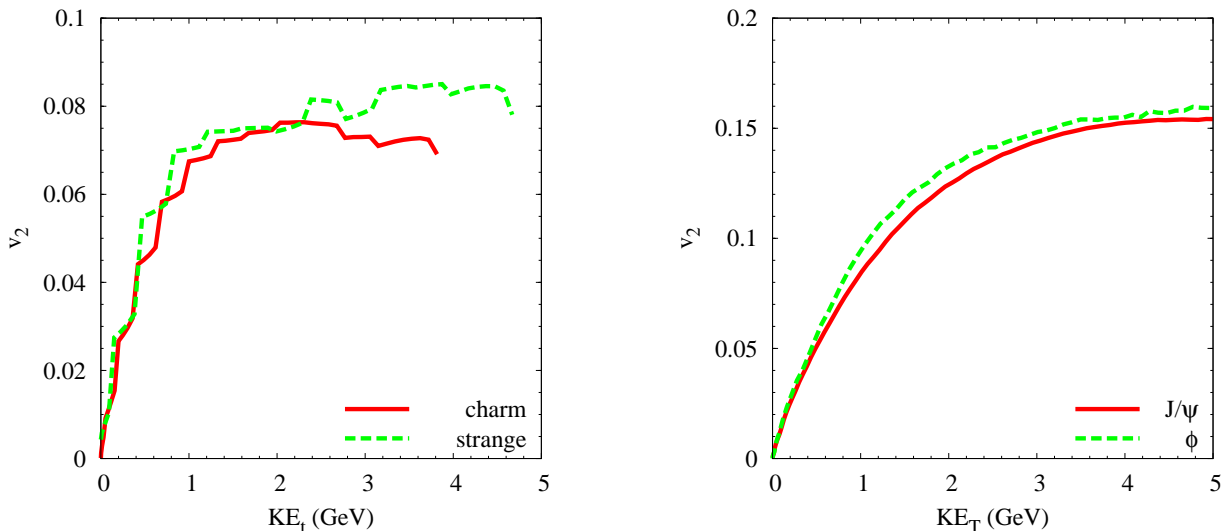
FIG. 6: (Color online) Elliptic flow coefficient, v_2 , as a function of transverse kinetic energy, K_{t,T} , for strange and charm quarks (left panel), as well as for \phi and J/\psi mesons (right panel).
