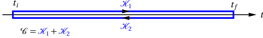
Figure 2.1: The Schwinger-Keldysh contour. The two branches are denoted with \mathcal{K}_1 (chronological branch) and \mathcal{K}_2 (anti-chronological branch). The ordering symbol \mathcal{T}_{\mathcal{C}} orders the operators with time arguments on the contour in the sense of the arrows from right to left. In the literature there are several conventions around. E.g. in the textbook [LL81] one finds the labels - and + instead of 1 and 2, respectively. In many papers the convention is the opposite. So use some care when studying the literature!
