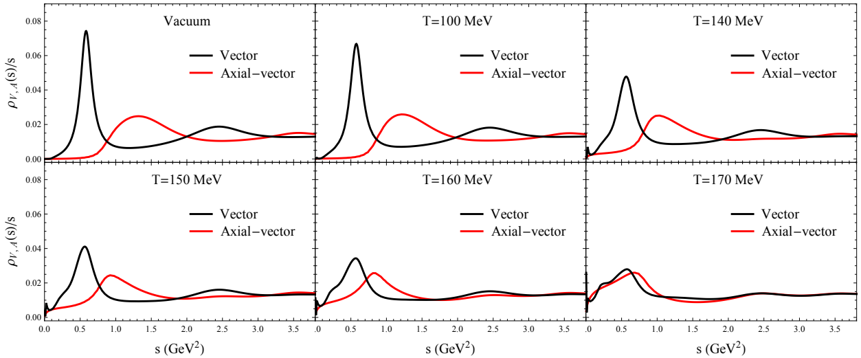
Fig. 2. Temperature progression (at \mu_B = 0 ) of the axialvector spectral function (red lines) as inferred from a simultaneous solution of QCD and Weinberg sum rules [12] using as input an in-medium vector spectral function from hadronic many-body theory [13] (black lines) and in-medium condensates as available from lattice QCD.
