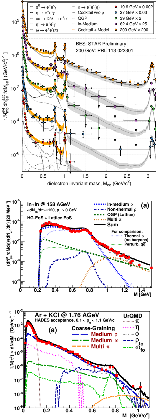
Fig. 3. Dilepton invariant-mass spectra from SIS-18 to top RHIC energies using the in-medium \rho spectral function of Ref. [13] for hadronic emission and in-medium q\bar{q} annihilation from the QGP. Top panel: excitation function measured in Au-Au collisions by STAR [17, 18], compared to predictions using a thermal fireball model [19] (Figure reprinted with permission from [17]). Lower two panels: NA60 data in In-In at CERN-SPS (middle panel) and Ar-KCl at GSI-SIS-18 (lower panel) calculated with the same dilepton emission rates implemented into a coarse-grained UrQMD approach [20, 21].
