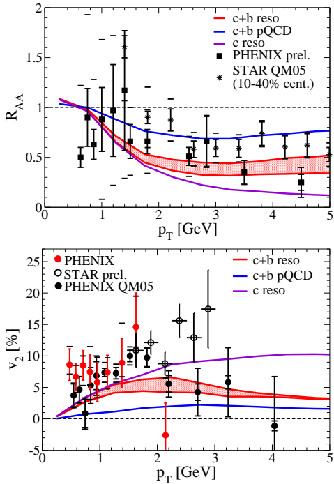
FIG. 3: Same as Fig. 2 but using HQ fragmentation only.
