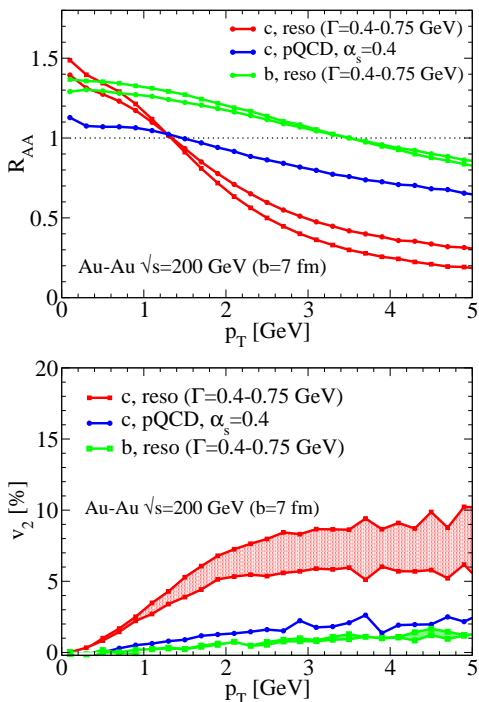
FIG. 1: Nuclear modification factor (upper panel) and elliptic flow (lower panel) of charm and bottom quarks in b=7 fm Au-Au( \sqrt{s}=200 GeV) collisions based on elastic rescattering in the QGP. Red (green) and blue lines are for c - ( b -) quarks with and without resonance rescattering, respectively, where the bands encompass resonance widths of \Gamma=0.4-0.75 GeV.
