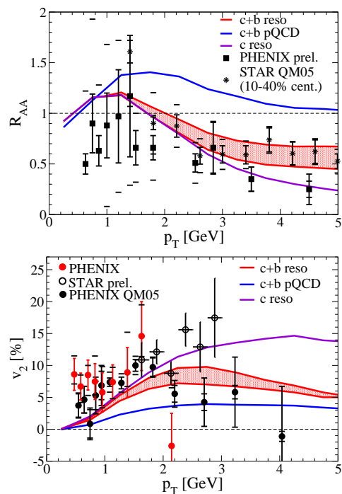
FIG. 2: R_{AA} (upper panel) and v_2 (lower panel) of semileptonic D - and B -meson decay-electrons in b=7 fm Au-Au( \sqrt{s}=200 GeV) using HQ coalescence supplemented by fragmentation (line identification as in Fig 1). The data [4, 6, 7, 8] are for minimum bias collisions, the R_{AA} from STAR [5] for 10-40% central collisions.
