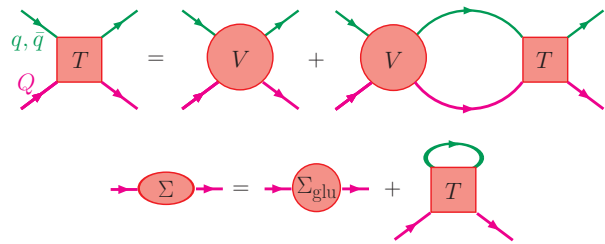
Fig. 1. (Color online) Diagrammatic representation of the Brueckner many-body scheme for the coupled system of the T -matrix based on the IQCD static internal potential energy as the interaction kernel and the HQ self-energy.
