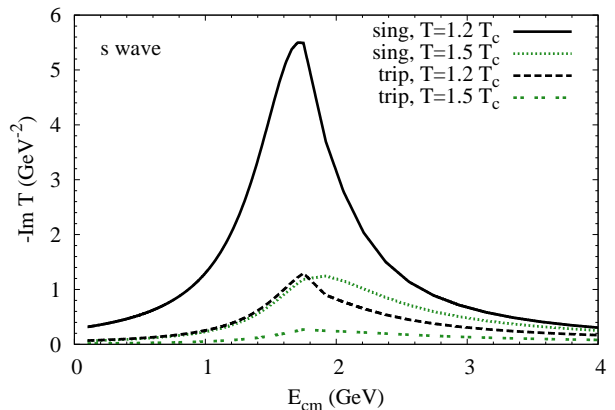
Fig. 2. (Color online) Imaginary part of the S -wave in-medium T matrix for c\bar{q} and cq scattering in the color-singlet and -antitriplet channels based on the parameterization of the IQCD potential energy by [Wo].
