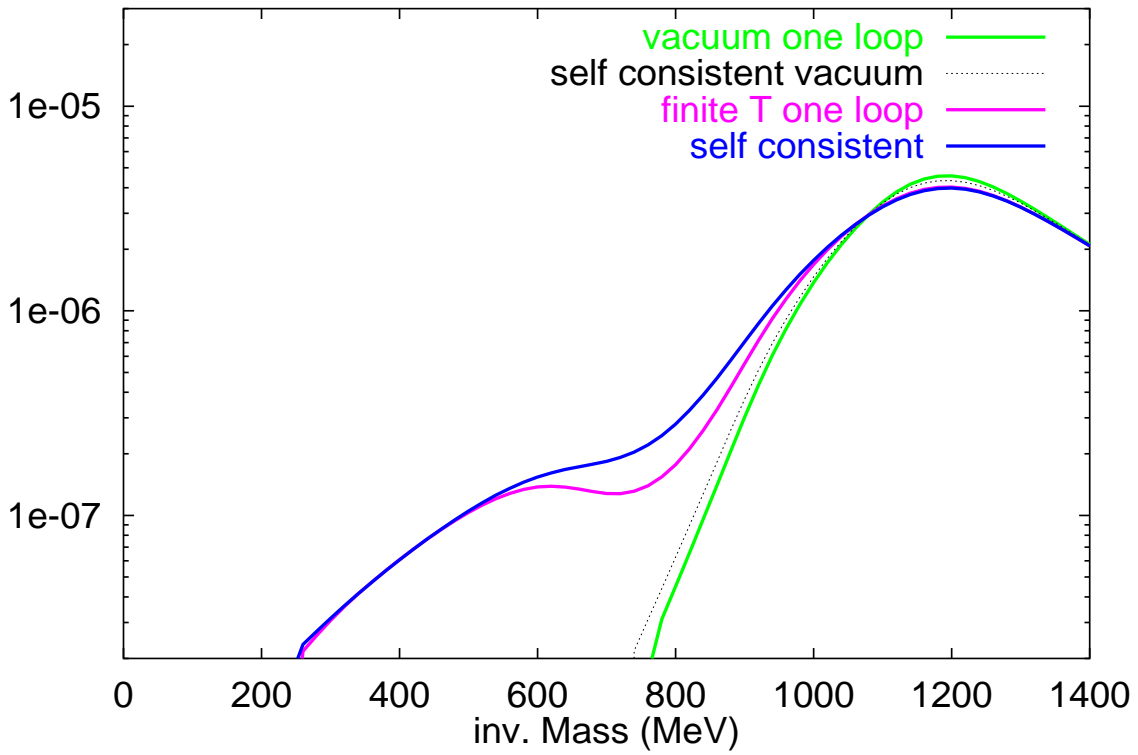
a1-Meson Spectral function, T=150 MeV
