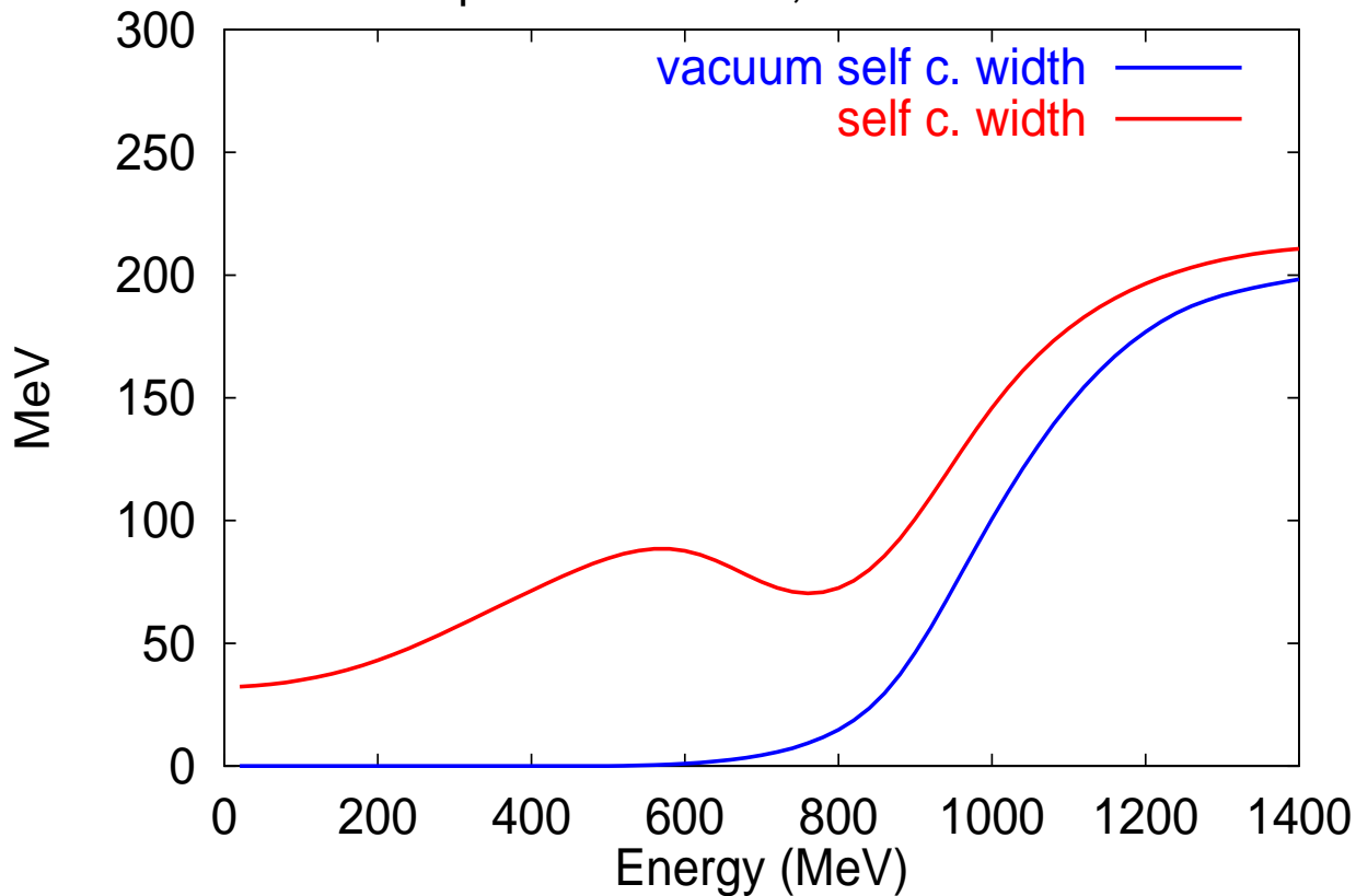
pi-Meson Width, T=300 MeV
