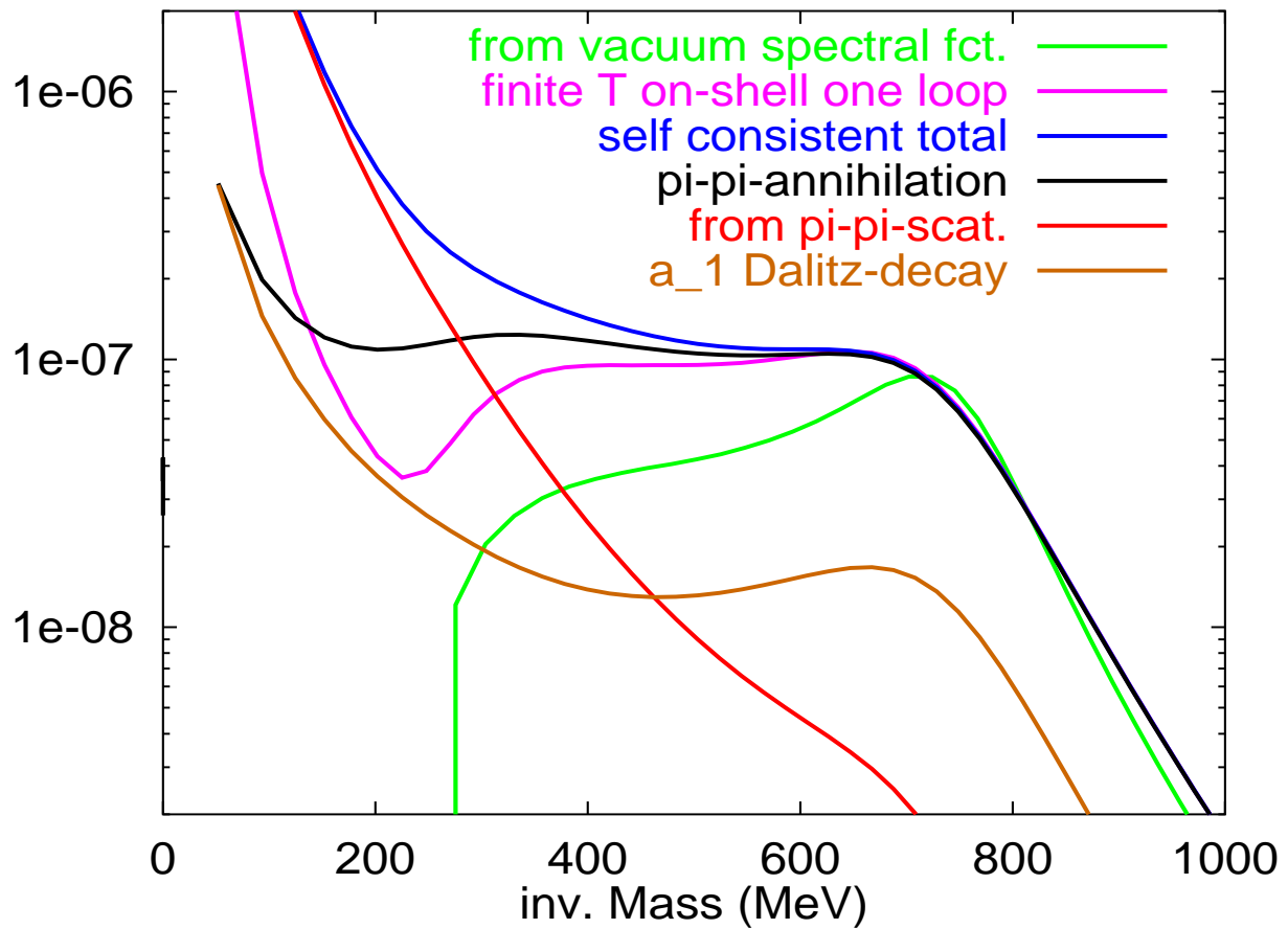
Dilepton rate (arb.units), T=150 MeV, p=150 MeV/c
