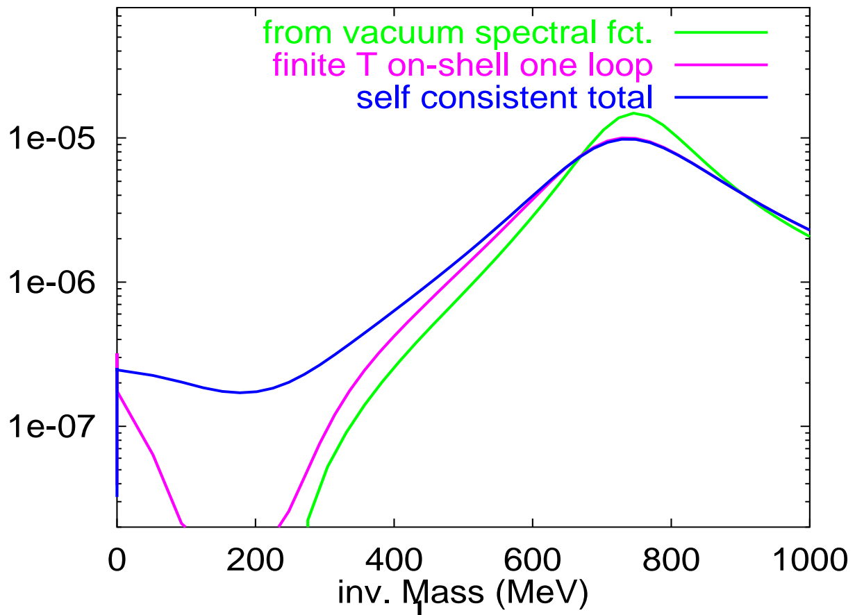
Rho-Meson Spectral Funct., T=150 MeV, p=150 MeV/c
