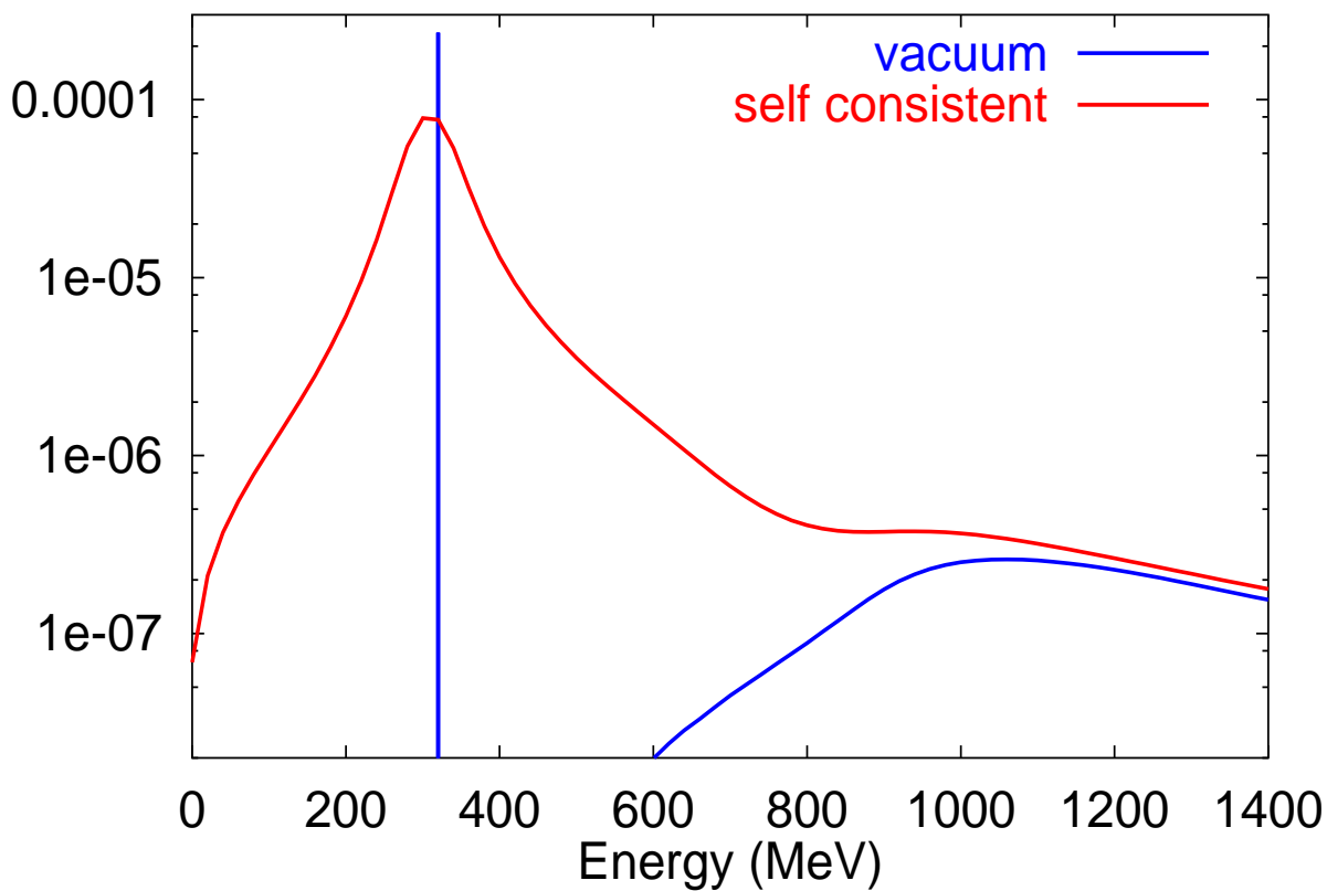
pi-Meson Spectral function, T=150 MeV; p=300 MeV/c
