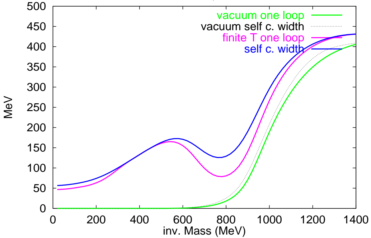
a1-meson width, T=150 MeV
