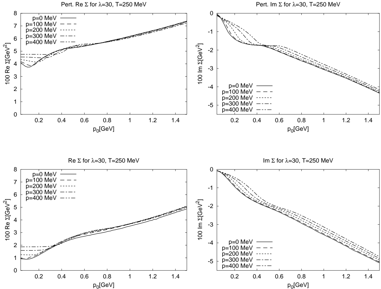
FIG. 6: Real (left) and imaginary part (right) of the perturbative (top) and the self-consistent self-energy for \lambda = 30 , m = 140\text{MeV} and T = 250\text{ MeV} as a function of p_0 for various 3-momenta. Note that the self-energies are multiplied by a factor of 100 in these plots!
