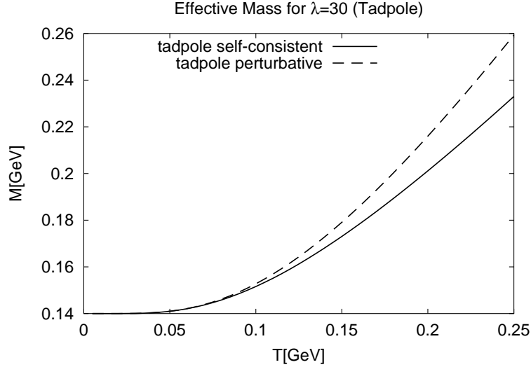
FIG. 1: The solution of the gap equation (24) compared to the naive, i.e., non-resummed one-loop perturbative solution. Both calculations are renormalized in the vacuum in the same way according to the on-shell conditions (9) with m = 0.14 GeV
