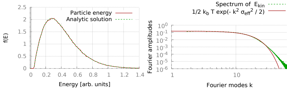
Fig. 1. (Color online) Left: The energy distribution of the quarks and anti-quarks follow the expected relativistic Maxwell-Boltzmann distribution f_q(E) \propto \exp(-E/T) , demonstrating the numerical stability of the kinetic equations as well as the validity of the principle of detailed balance. Right: The spectrum of the kinetic energy density of the mean field, \phi^2/2 . For low k (long wavelengths) the distribution follows the expected equipartition theorem for a classical field. At higher energies the finite interaction volume encoded in the finite width of the Gaussian wave packets leads to an effective cut-off.
